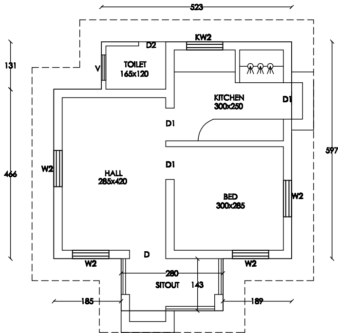
FLOOR PLAN FLOOR AREA: 444.00 Sqft OPTION-1
